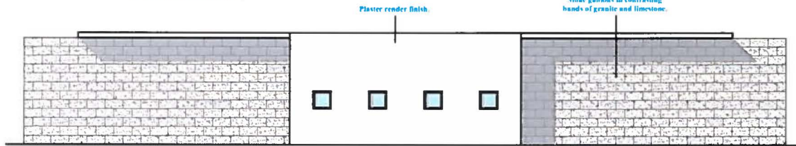
REAR ELEVATION - 1 : 100
